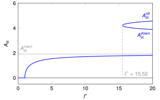
Fig. 3. Variation of the nontrivial solutions of (26) as \Gamma is increased. Only the trivial solution exists for \Gamma < 1 . Then, the primary branch is the unique nontrivial solution for 1 < \Gamma < 15.52 . This primary branch of solutions, which exists for all \Gamma > 1 , increases monotonously but has a horizontal asymptote A_{st}^{\max1} = 1.91 . New nontrivial solutions (secondary branch) emerge for \Gamma > 15.52 . The bifurcation analysis shows that the microwave envelope \mathcal{A} undergoes a pitchfork bifurcation at \Gamma = 1 , which corresponds to a Hopf bifurcation for the microwave voltage variable V . The same analysis also shows that \mathcal{A} undergoes a saddle-node bifurcation at \Gamma = 15.52 (emergence of two new fixed points, one being stable and the other one unstable). The system, therefore, starts in that case to evidence hysteresis, with two stable solutions (lowest and highest amplitudes) and an unstable solution (corresponding to the intermediate amplitude). As \Gamma is further increased, the system undergoes saddle-node bifurcations any time a new branch of paired solutions emerges.
